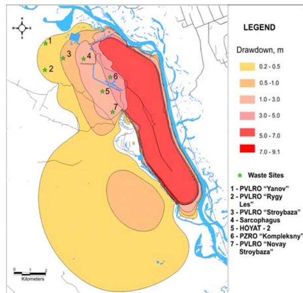
GROUNDWATER DRAW-DOWN FROM LAGOON DRAINING
